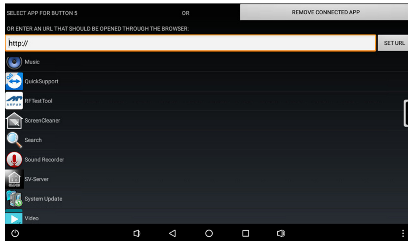
Fig. 8: App shortcut
