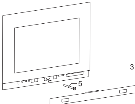
Fig. 3: Locking screw under design cover
