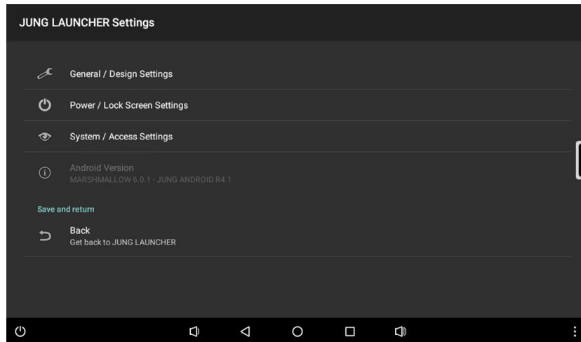
Fig. 4: Settings
