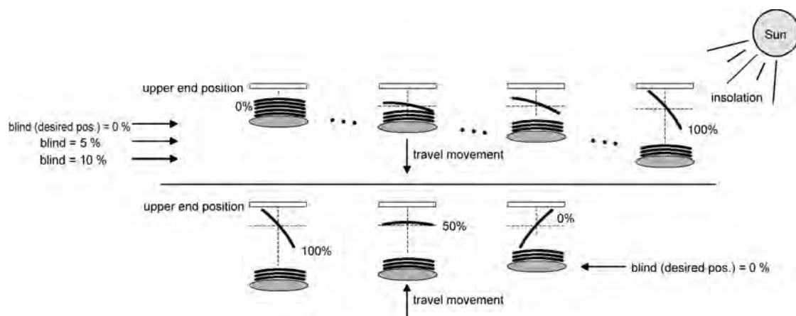
Figure 19: Example of slat positioning with the Venetian blind in upper end position (typical of slat type 1)
