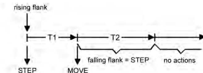
Figure 10: Operation concept "short - long - short"
