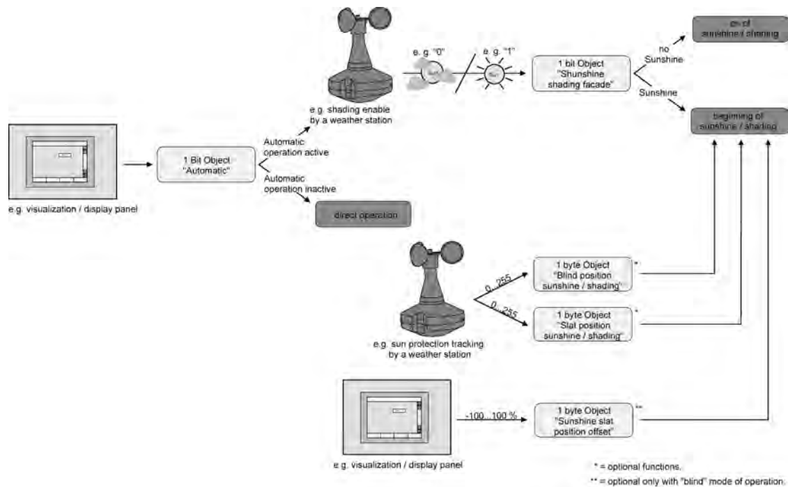
Figure 25: Schematic diagram illustrating the extended sun protection configuration (for reasons of simplicity without disabling functions)
