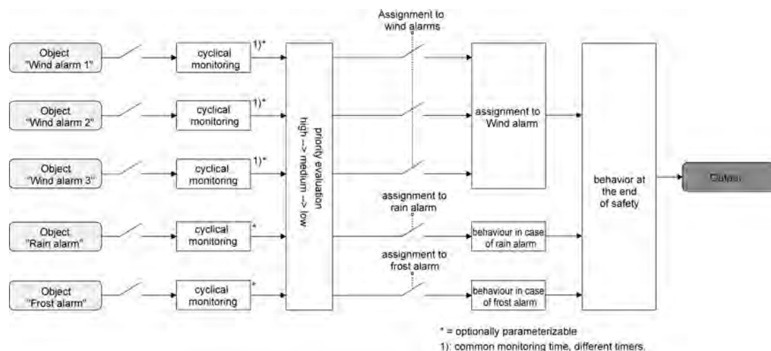
Figure 21: Function diagram of the safety function
