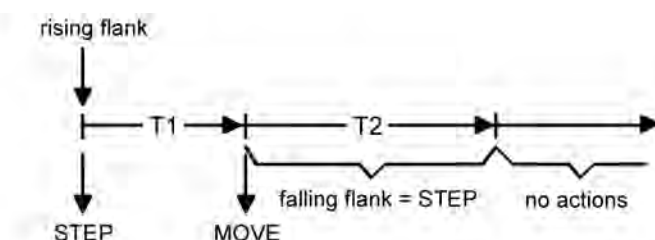
Figure 9: Operating concept "Short - long - short" when inputs 1 and 2 have an internal impact
