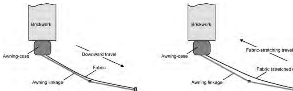
Figure 35: Fabric stretching in an awning
