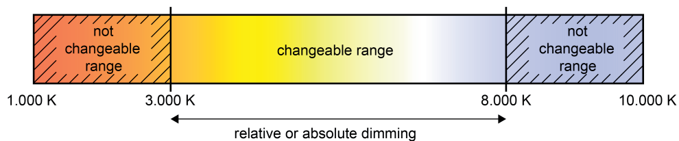
Figure 38: Automatic adjustment of the colour temperature to the set brightness Example with limited brightness and colour temperature range
