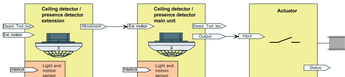
Figure 36: Application example without twilight level evaluation in the main unit and extensions for output functions "temperature value transmitter" and "operating mode room temperature controller"
